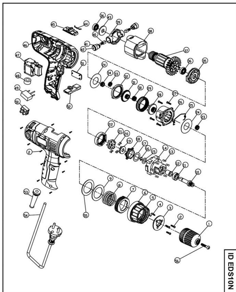
Exploded view for ID EDS10N
