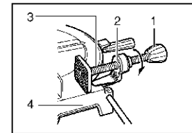
1. Vise knob 2. Projection 3. Vise shaft 4. Base
