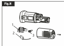
1.Brush Holder 2.Carbon Brush 3.Coil Spring
